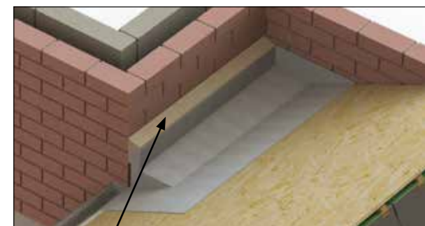
59mm timber packer, lead flash over into tapered box gutter.
