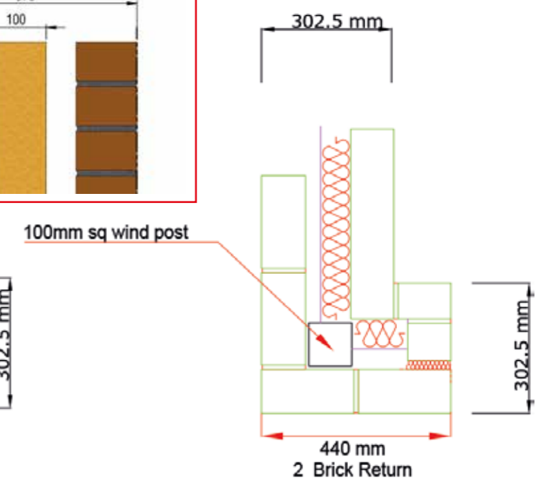
Minimum Brick Return with Wind Post
