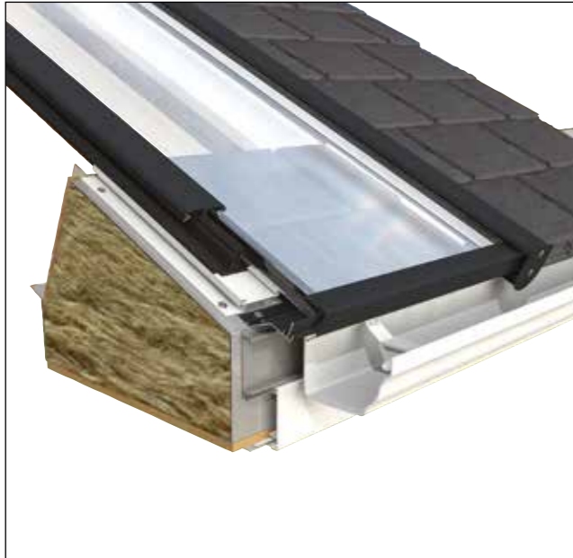
Ridge solid to glass
