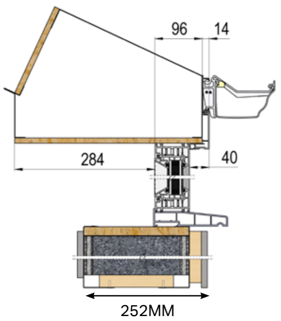
HUP! ON FRAME WITH 40MM SOFFIT
