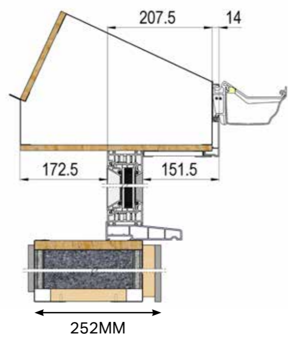
HUP! ON FRAME WITH 151.5MM SOFFIT
