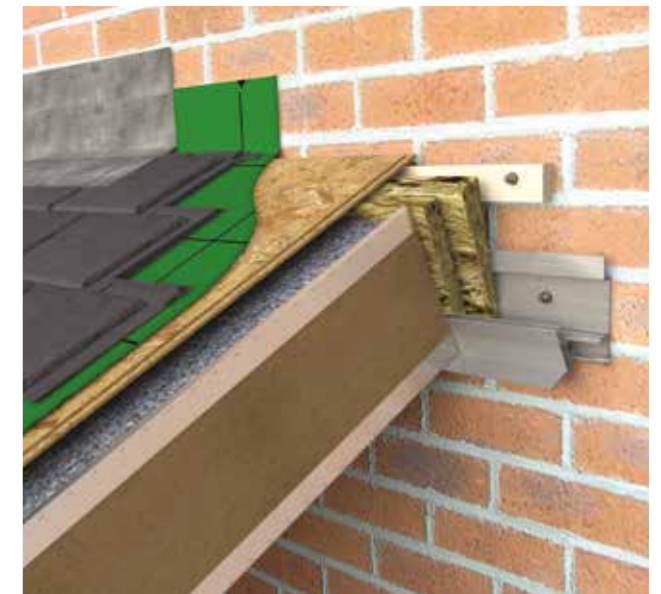
Gable extended
