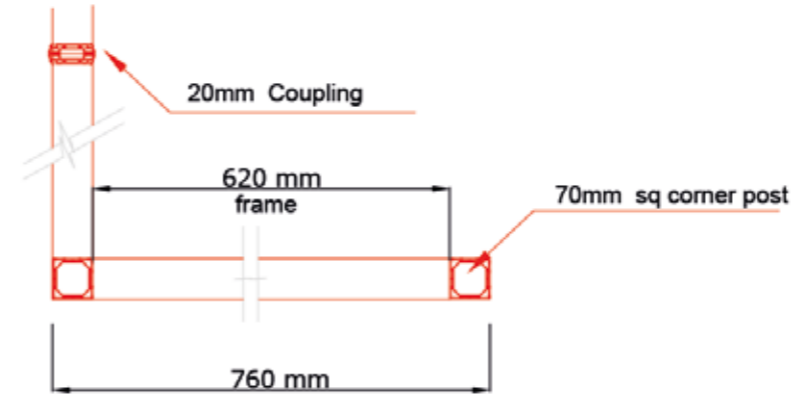
Minimum Frame Return Detail (When adjacent/in line with 4m unsupported span)
